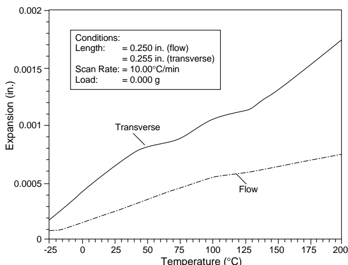
Figure 2 Dimensional change of 40% glass-reinforced Fortron® PPS
