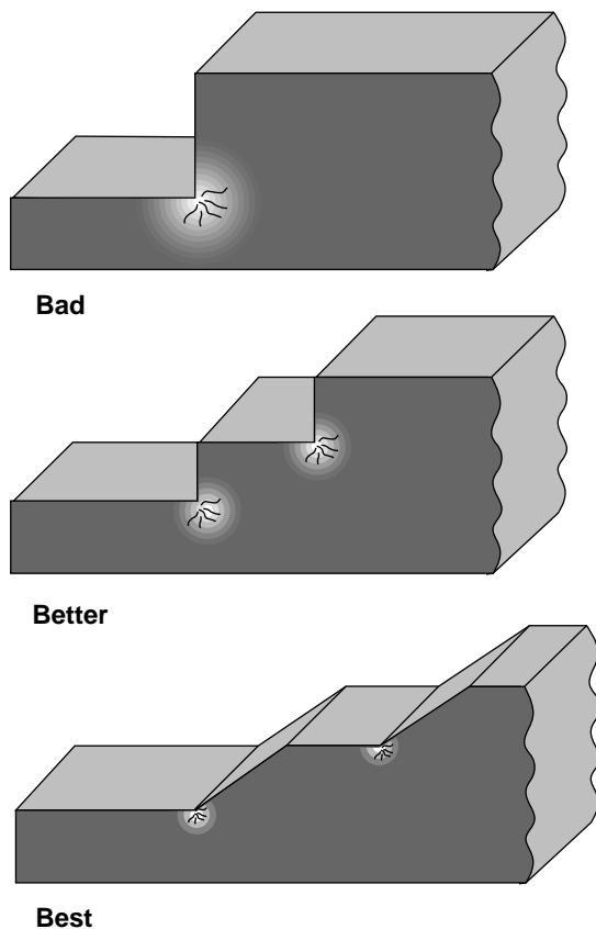
Figure 1 Design of nominal wall from thick to thin sections
