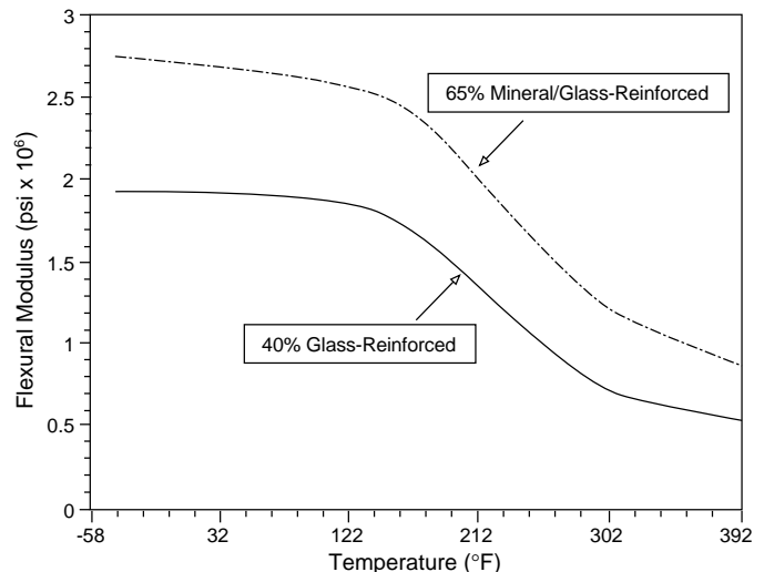
Figure 4 Temperature dependence of flexural modulus
