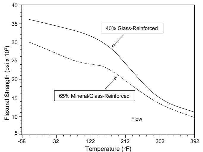
Figure 3 Temperature dependence of flexural strength
