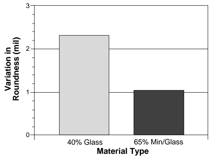
Figure 11 Warpage with respect to roundness of a hole
