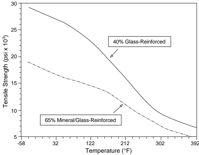
Figure 5 Temperature dependence of tensile strength at break
