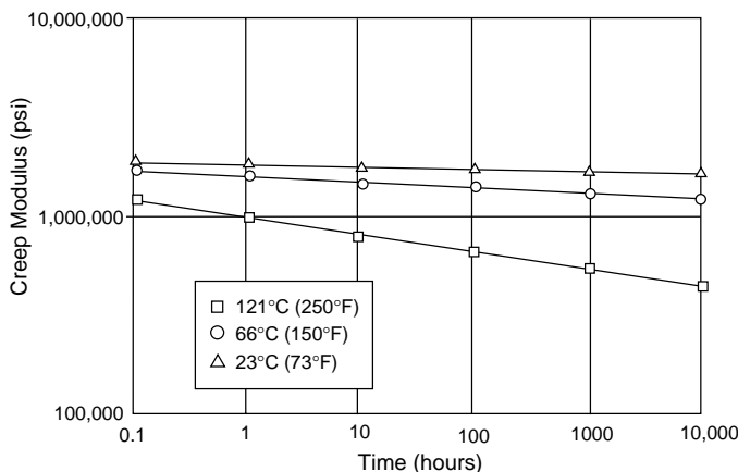
Figure 7 Creep modulus in three-point bending of 40% glass-reinforced Fortron® PPS; stress = 5000 psi
