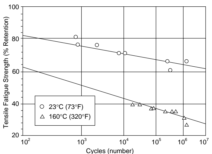
Figure 13 Fatigue resistance of 65% mineral/glass-reinforced Fortron® PPS
