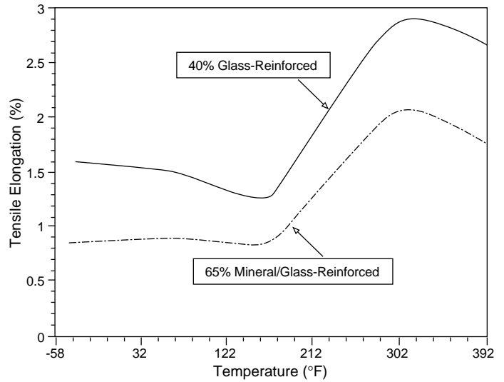
Figure 6 Temperature dependence of tensile elongation at break
