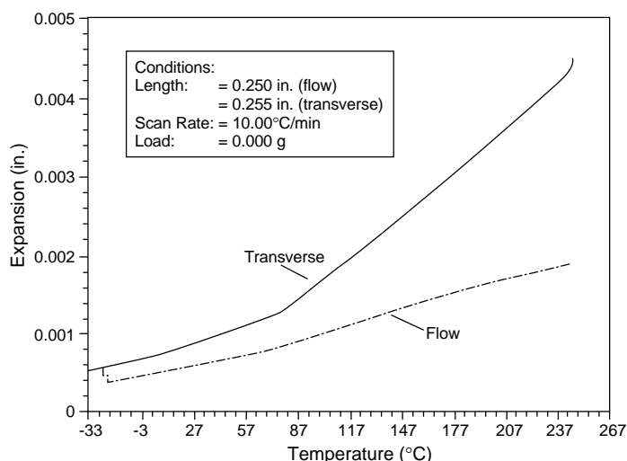
Figure 1 Dimensional change of mineral/glass-reinforced Fortron® PPS
