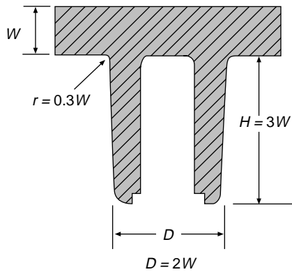
Figure 3 Design of a self-tapping screw boss
